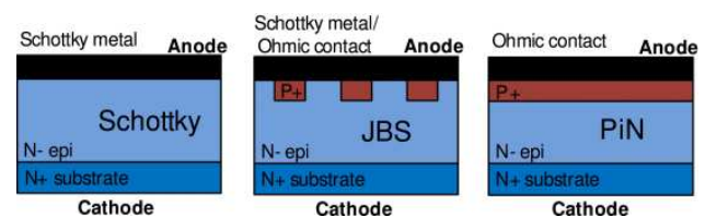
Fig. 2. Three basic SiC diode structures.
