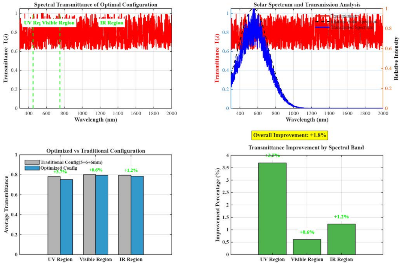
Fig. 8 comparison of average transmittance between optimized configuration and traditional configuration (original)
