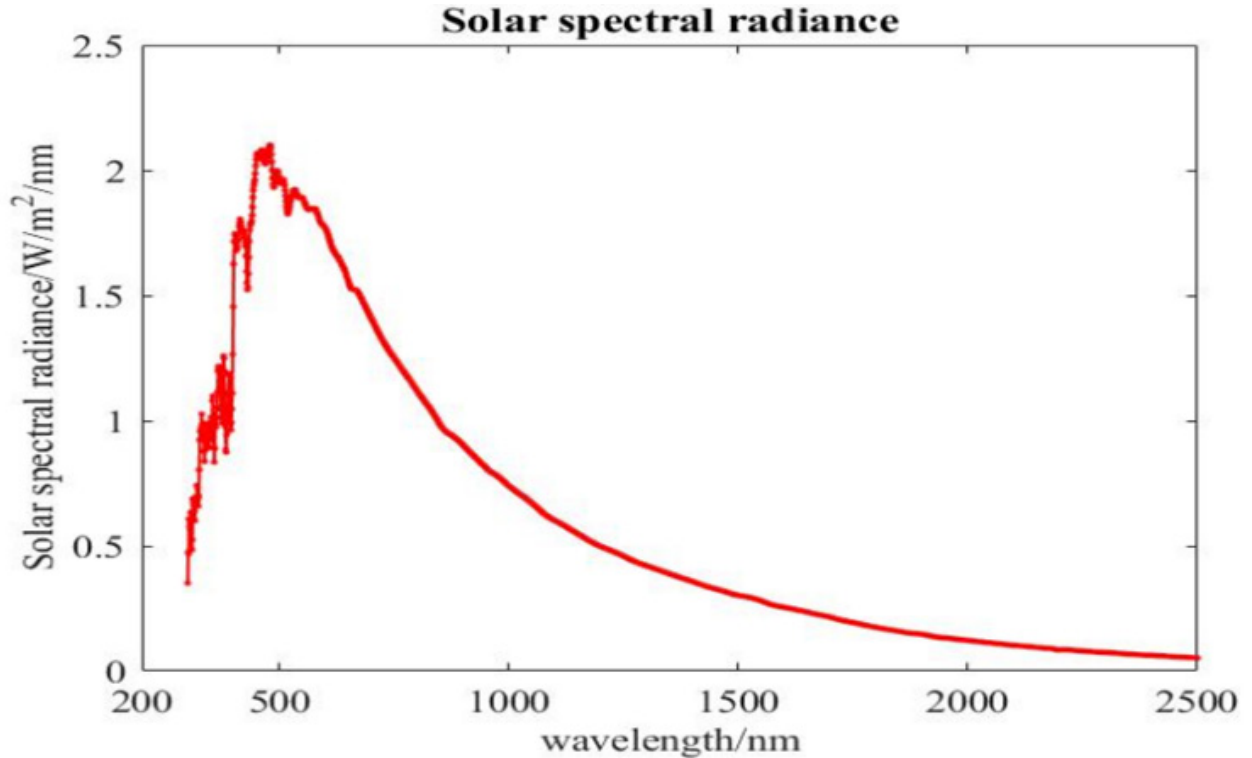
Fig. 1 Standard solar spectral irradiance data (AM 1.5) [11]
