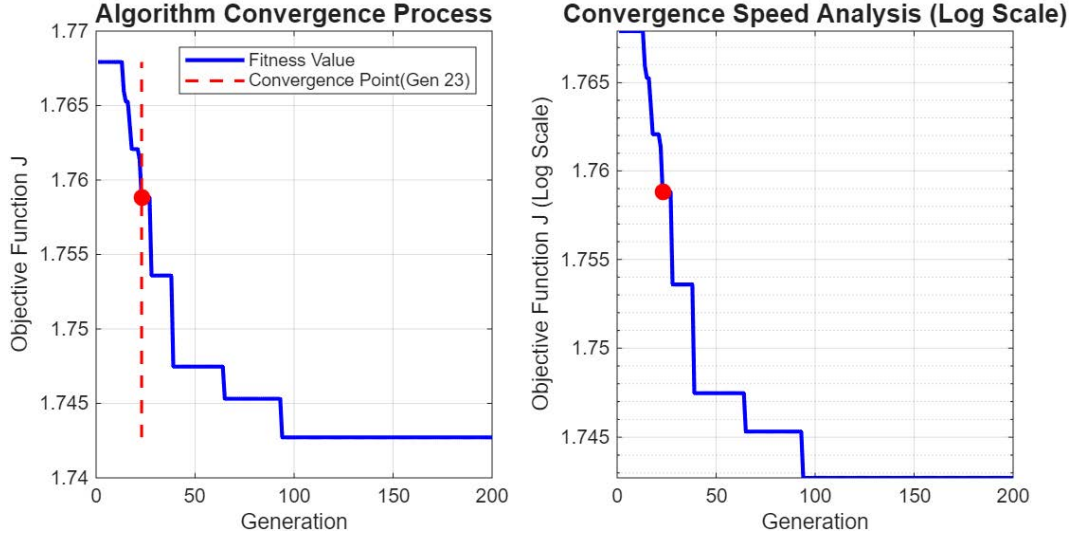
Fig. 6 Evolutionary convergence curve of quantum genetic algorithm (original)
