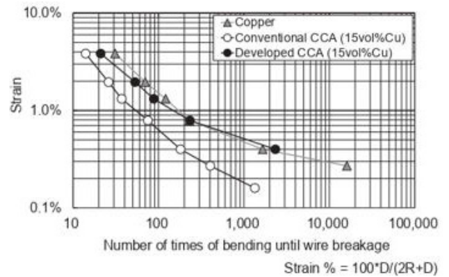
Fig. 1 Evaluation of developed CCA wire's resistance to bending fatigue fracture [11]
