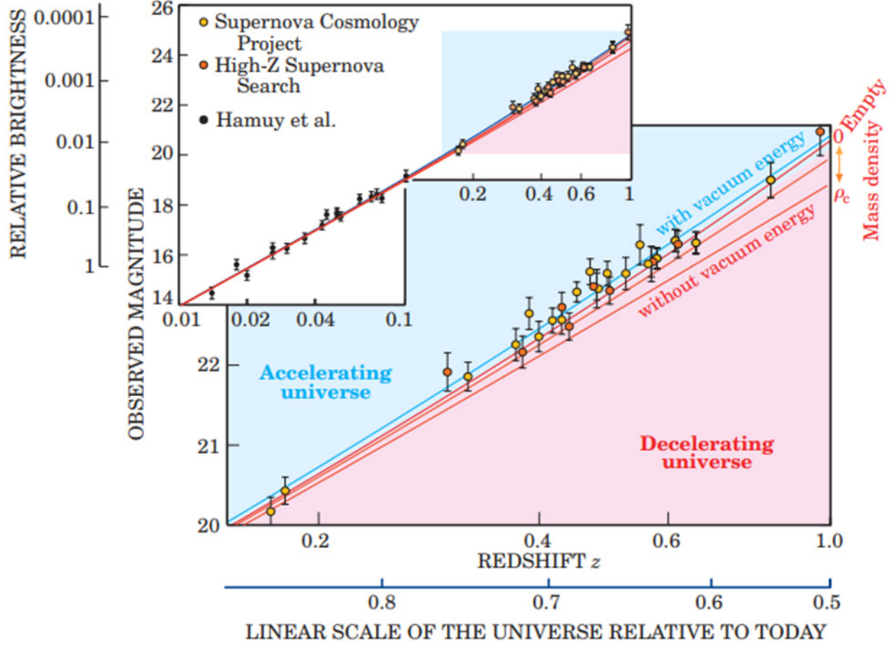
Figure 1: The observed luminosity from the official publication of Supernova Cosmology Project [1].
