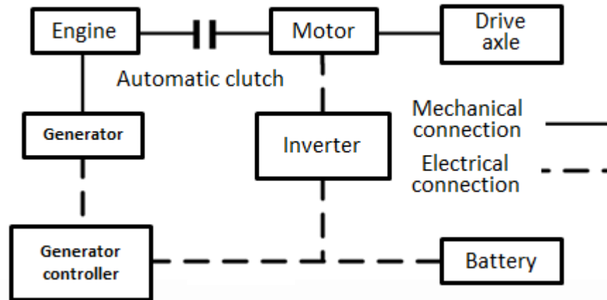
Fig. 3 Power-split hybrid system [13].
