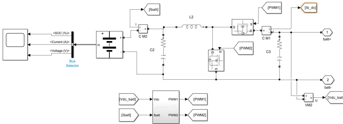
Fig. 9 Energy storage system
