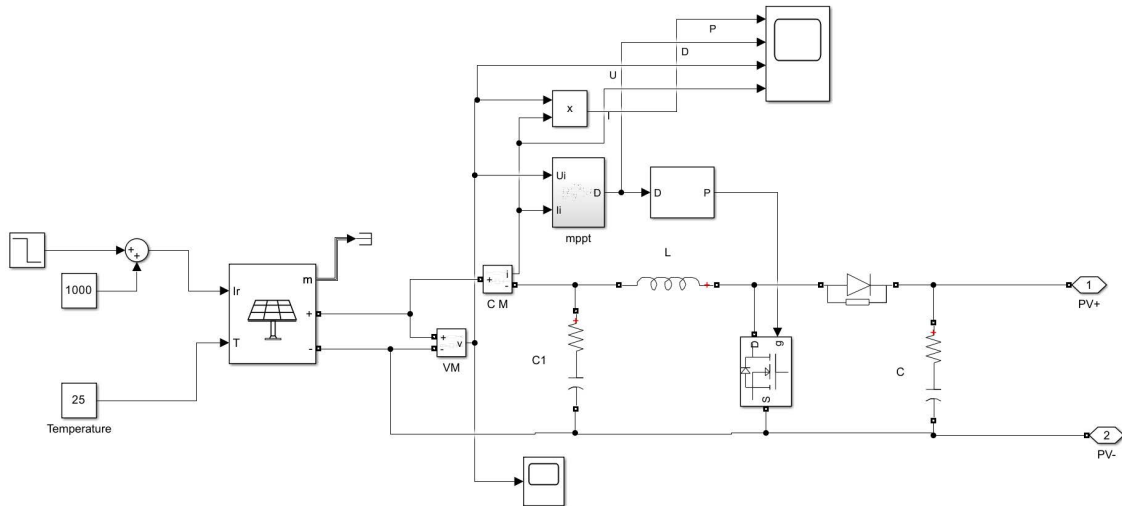
Fig. 3 Photovoltaic system
