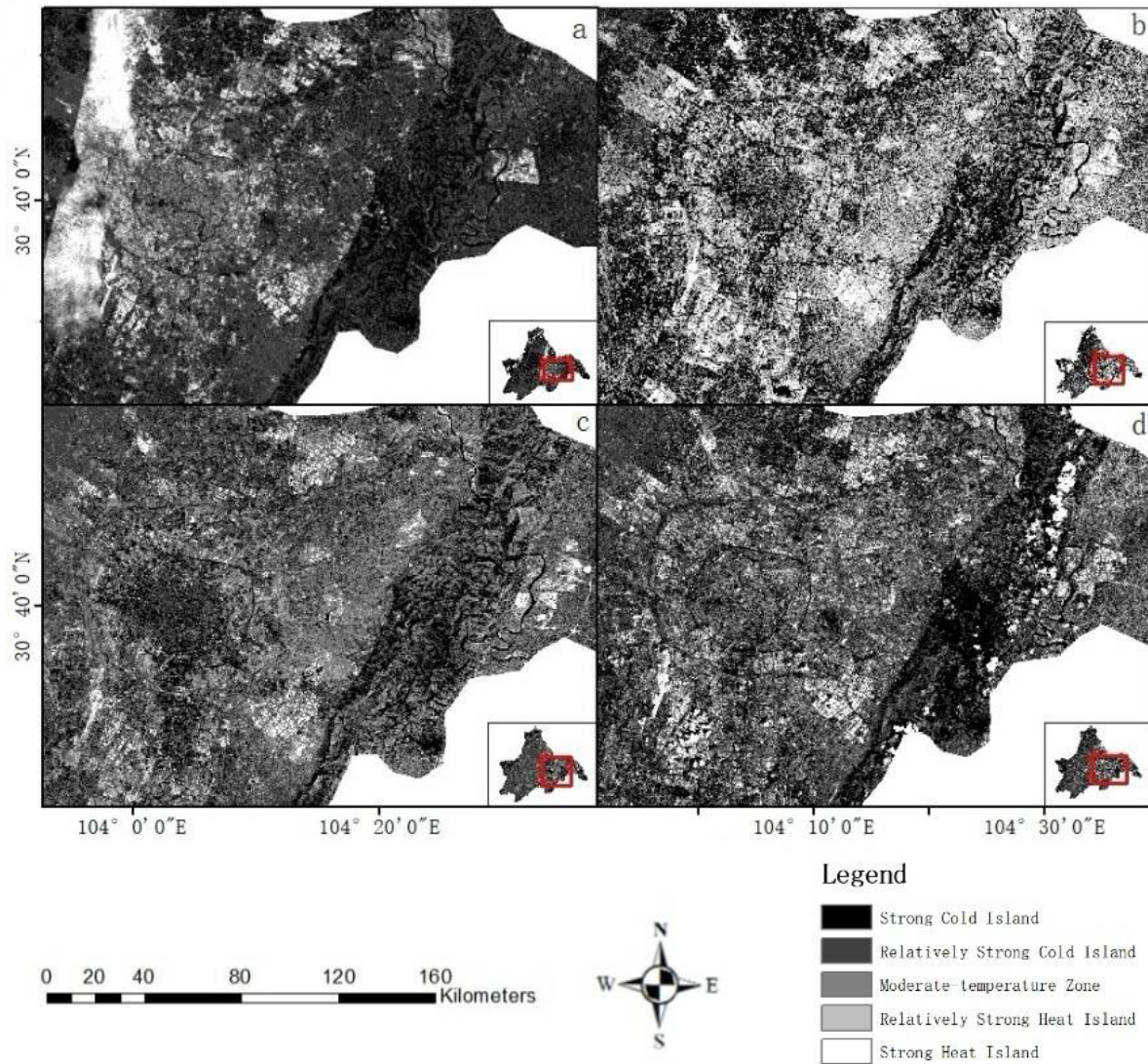
Fig.1 Land surface temperature inversion plot (a: urban land surface temperature in 2014; b: urban land surface temperature in 2018; c: urban land surface temperature in 2021; d: Urban surface temperature in 2024)
