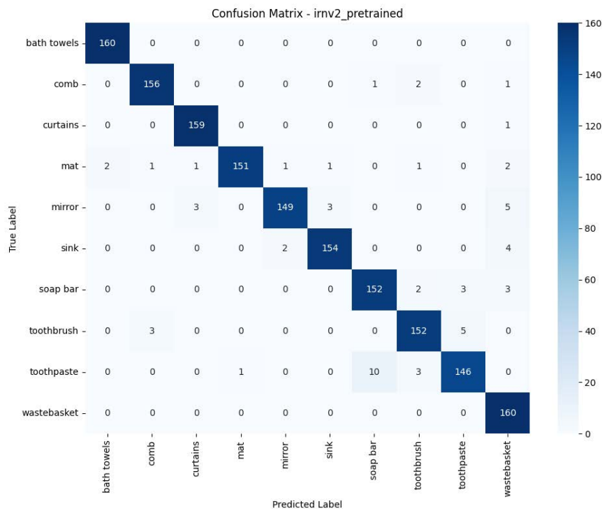
Fig. 5 Confusion matrix – InceptionResNetV2 (Pretrained) (Picture credit : Original)
