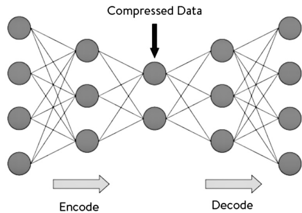
Figure 1. Autoencoders architecture
