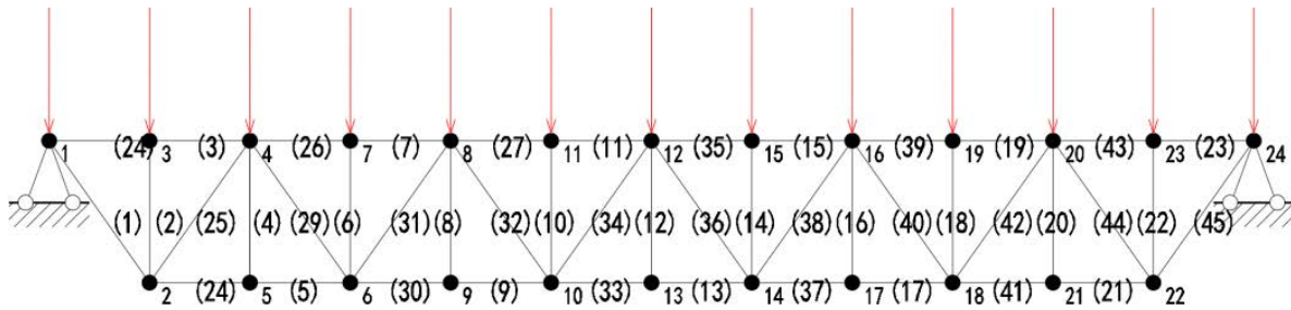
Figure 3: Optimization of front overhead truss bridge.
