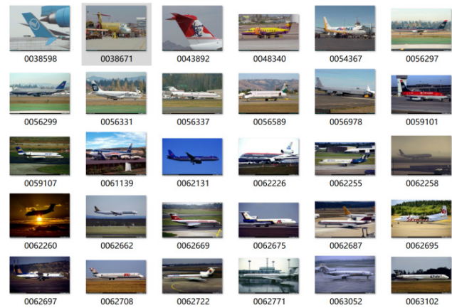
Fig. 1 FGVC-Aircraft dataset [5].
