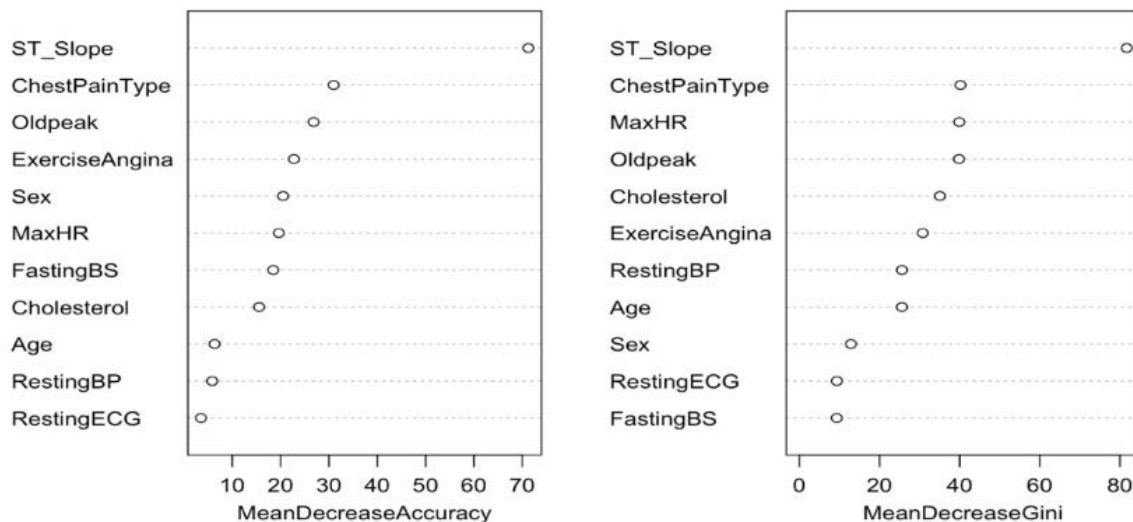
Fig. 6 Random Forest feature importance (Photo/Picture credit: Original).
