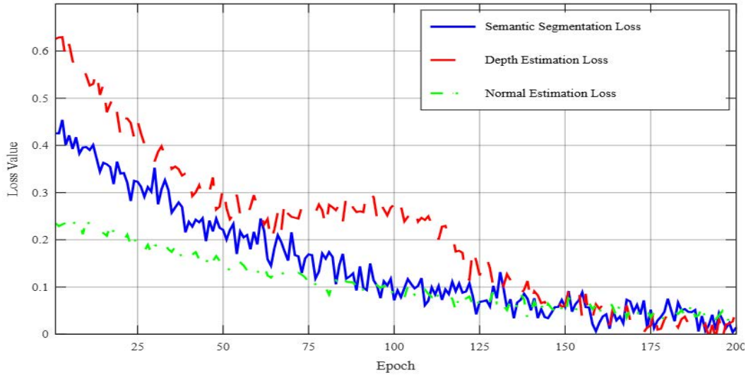
Fig. 3 Loss plot.
