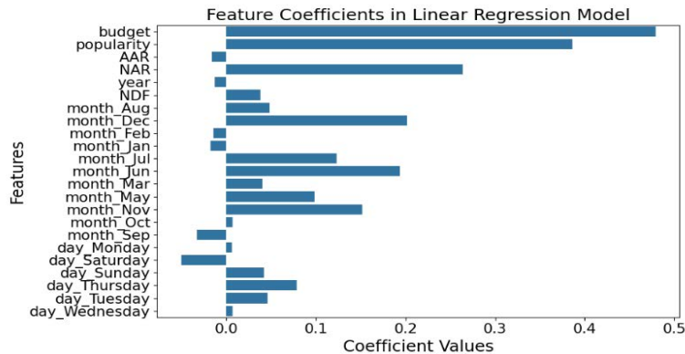
Fig. 4 Linear Regression Feature Coefficients (Picture credit: Original)
