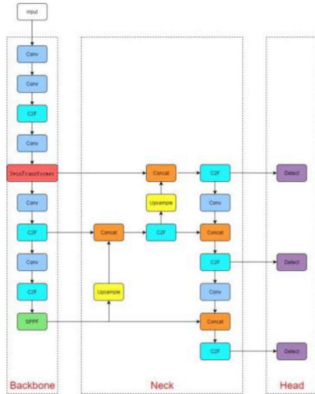
Fig.10 YOLO v8n-swin convolutional network
