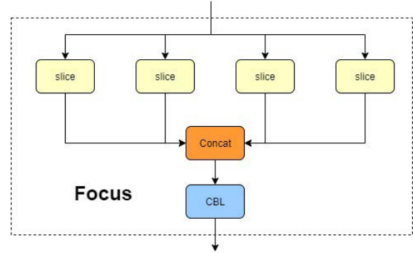
Fig.2 The convolutional network of the Focus model
