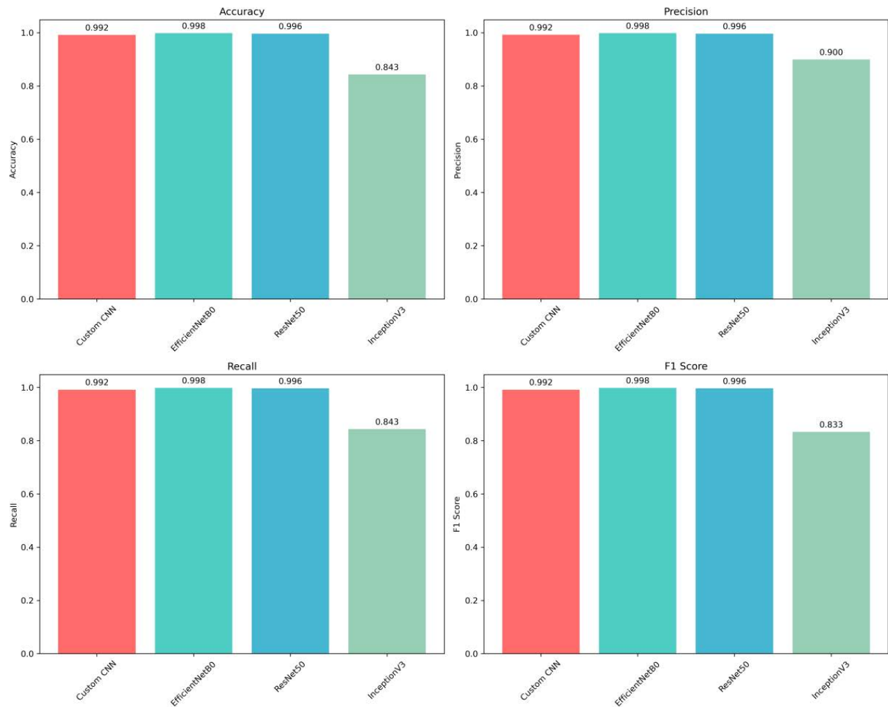
Fig. 1 Comparison of each model's overall performance in terms of F1-score, recall, accuracy, and precision (Picture credit : Original)
