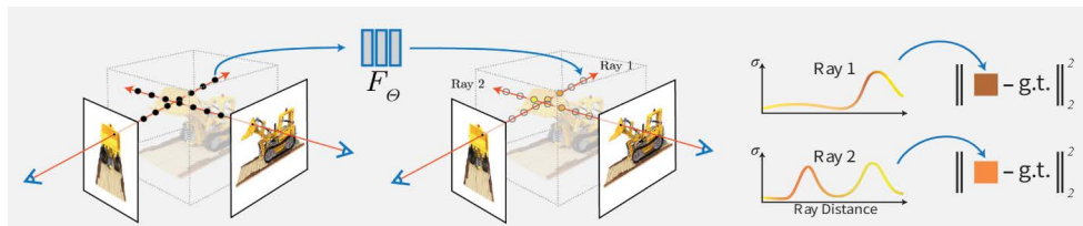
Fig 1. Schematic diagram of the basic principle of NeRF technology
