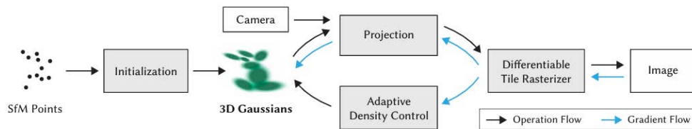
Fig 2. Linear block diagram of the principle of 3DGS technology
