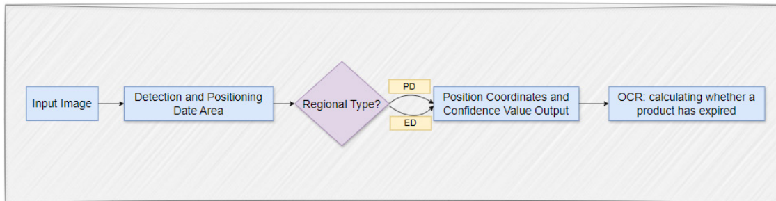
Figure 13. End to end recognition process
