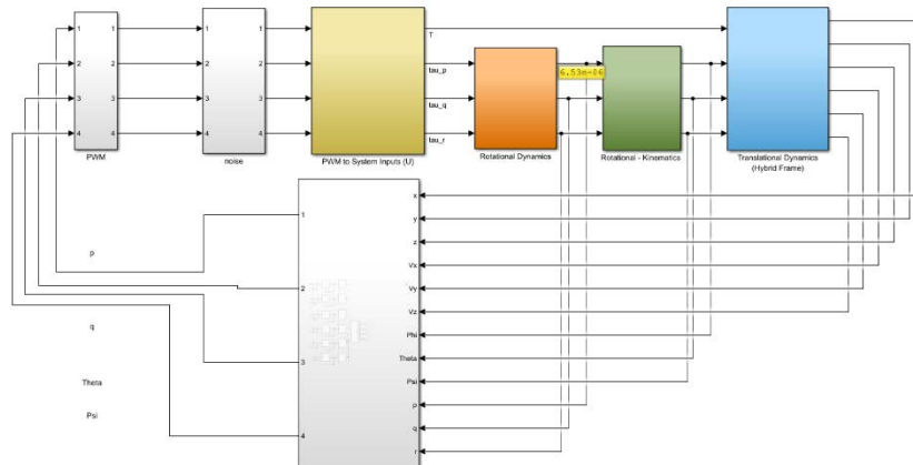
Figure 3 Quadrotor UAV PID Controller Simulink Model.
